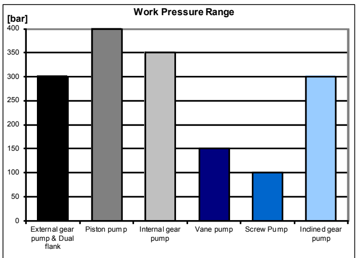
Above: comparison between the different fields of use of other kinds of volumetric pumps.
