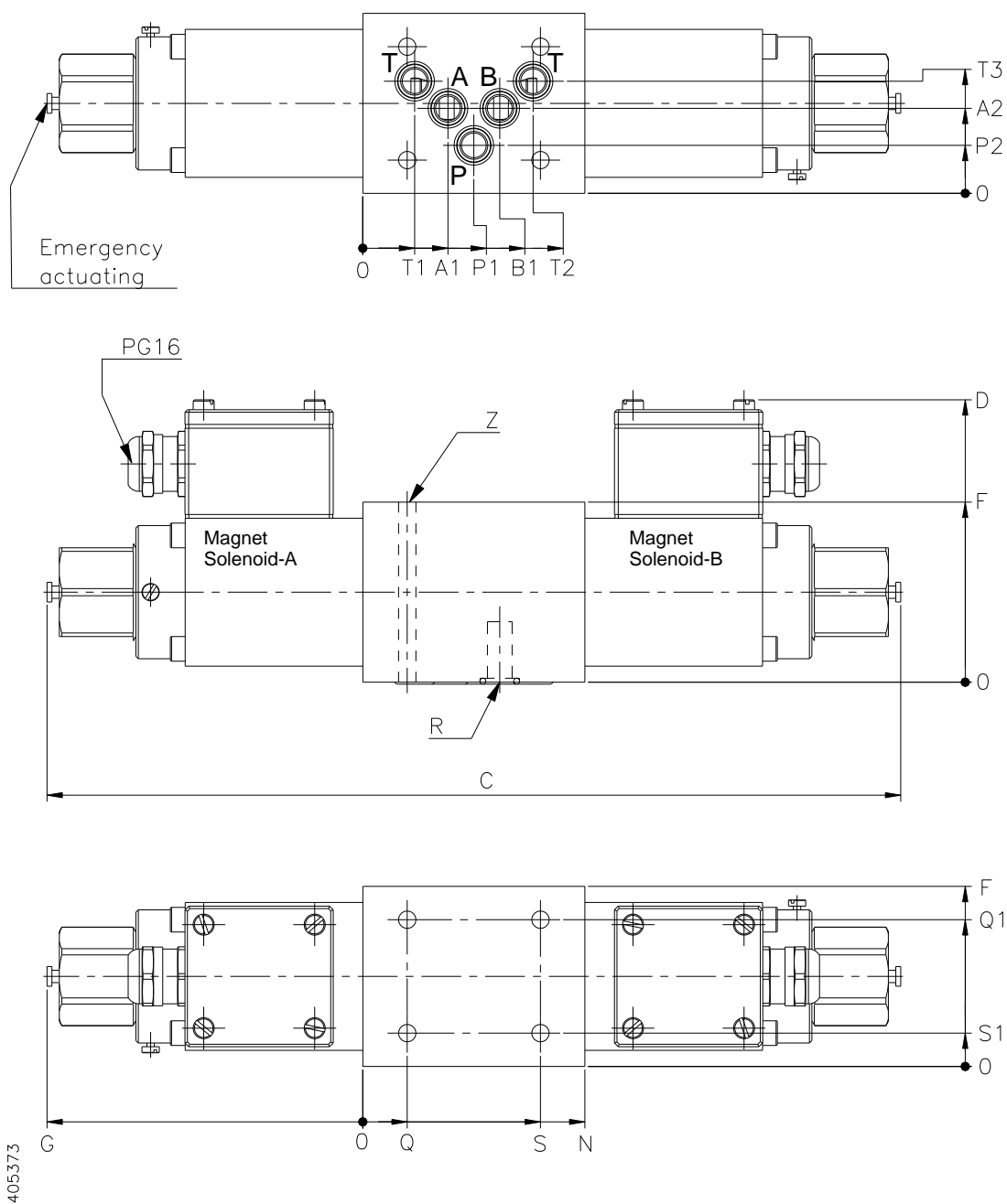
Figure 2 1STB4432 Dimensions
