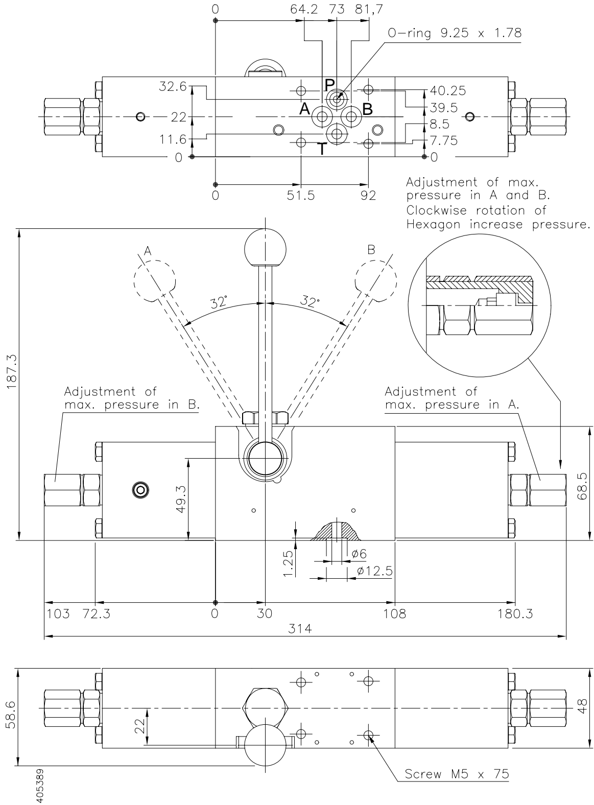
Figure 2 1FGB Dimensions
