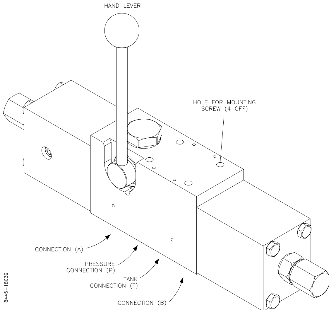
Figure 1 1FGB General Arrangement
