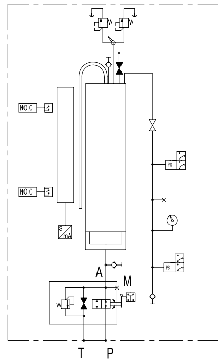
HYDRAULIC DIAGRAM
