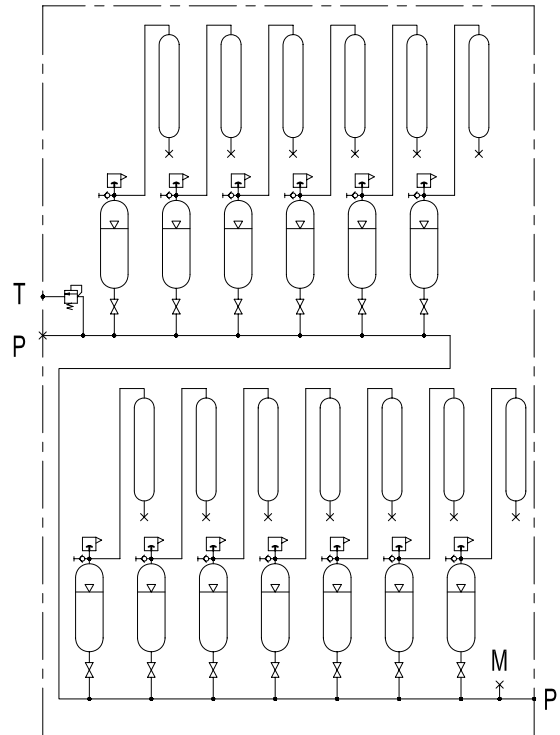
HYDRAULIC DIAGRAM
