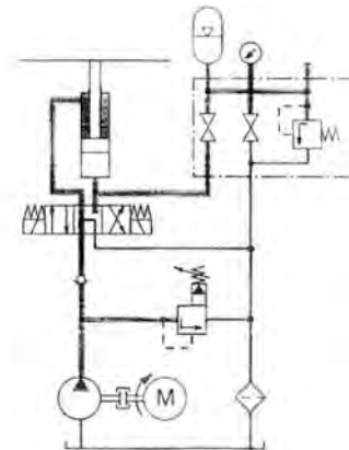
Fig. 1.3m: leak compensation
