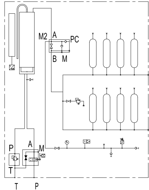
HYDRAULIC DIAGRAM
