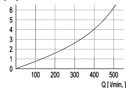
BC32 non-return valve ΔP [bar]
