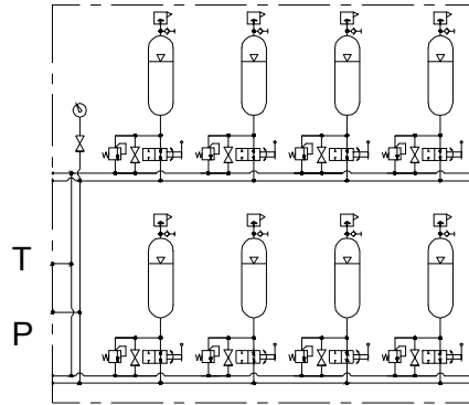
HYDRAULIC DIAGRAM
