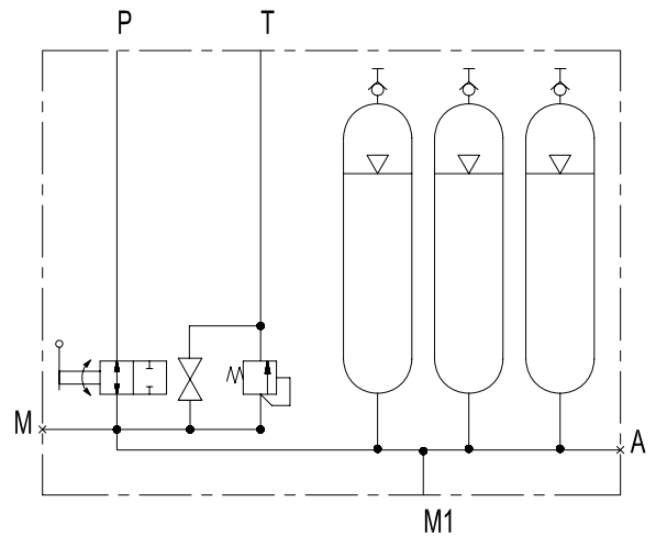
HYDRAULIC DIAGRAM
