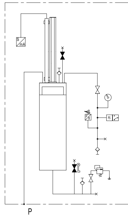
HYDRAULIC DIAGRAM
