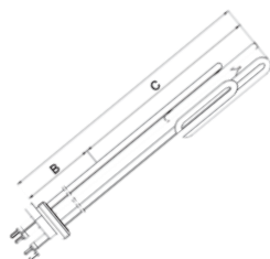
Heater 230V 1000W Art.nr: 690031
