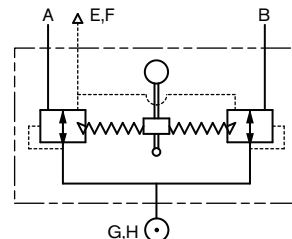
CIRCUIT SYMBOL LEVER CONTROL VALVE
