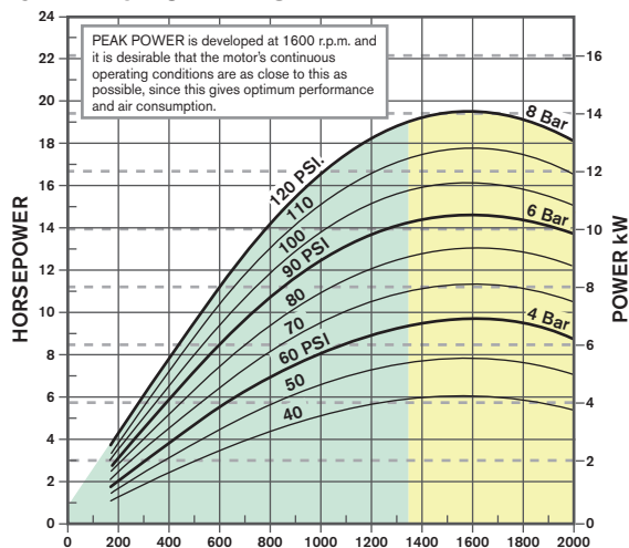
GRAPH 3 POWER - SPEED
