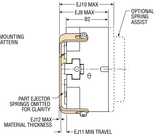
PART EJECTOR EXTENDED
